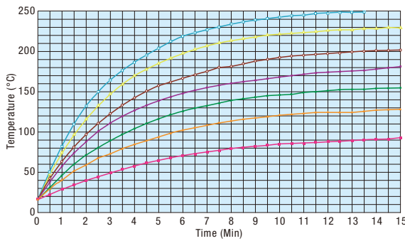
- Actual Measurement Data: Time of Increasing Temperature for Each Electric Power (Electrical Power Density)
