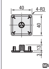
HFCB8-4040 (Screw Fixing Type)
