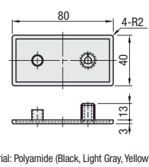
HFCB8-4080 (Screw Fixing Type)
