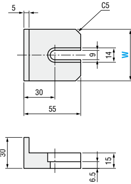
Side gauge FLOSG
