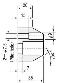
Rear gauge FLORG
