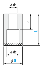
Preload pin FLAP
