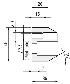
Side gauge FLOSG
